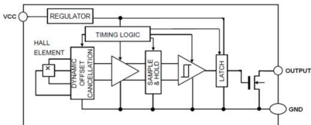
Figure 3, Block Diagram of AS1916C
