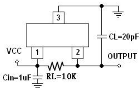
Figure 1, Typical Application Circuit of AS1916C
