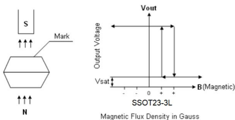
Fig 4, Magnetic Operation Characteristic of AS1916C
